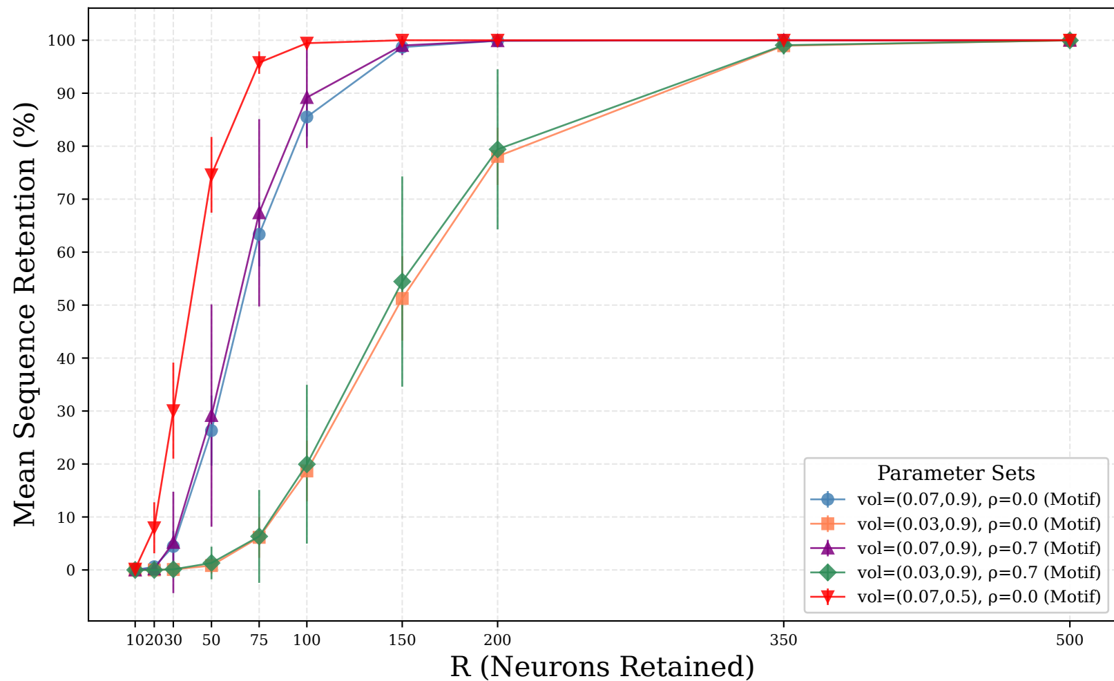
Mean Sequence Retention vs Neuron Threshold (R) with R Thresholds for 50% Retention
